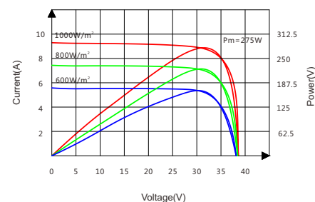
Current-Voltage&Power-Voltage Curve(275W)
